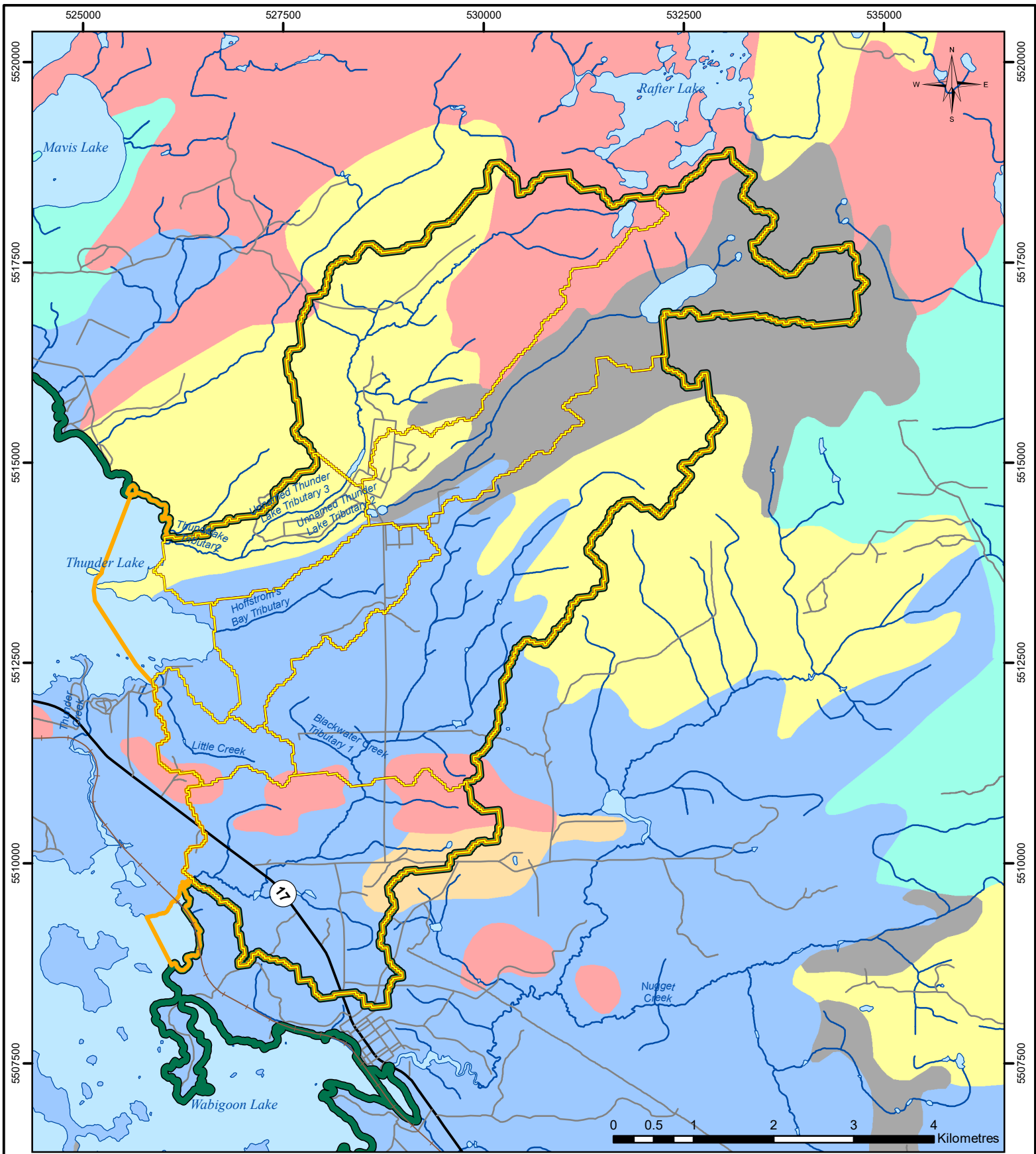
Figure 5.8.4.3-1 Surficial Geology
